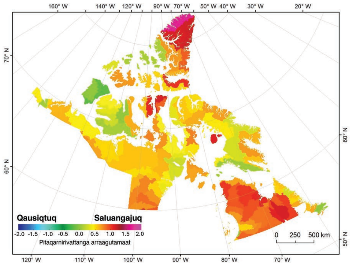
Ajjinguaq 6: Nunannguaq Nunaup Qaanganiitut Imaqarniujut (2004-2023)
