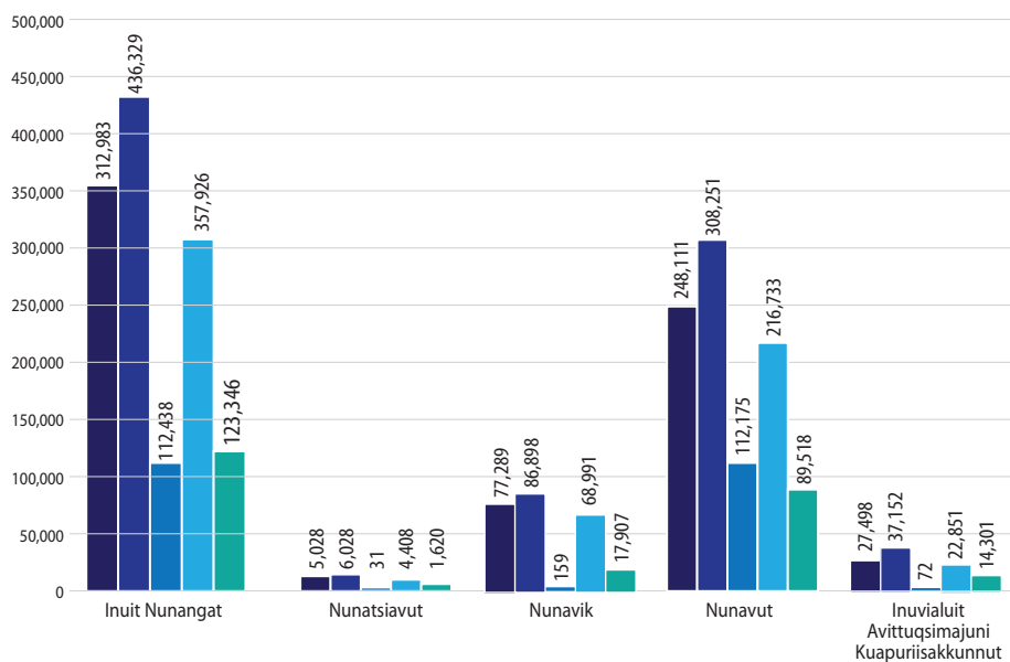
Ajjiinguaq 5: Nunaup Qaanganiinginnaqtut Imatsiat, Aujuittut asingillu nunami qaujisaqtauju Inuit Nunanganni (km 2 -ni)
