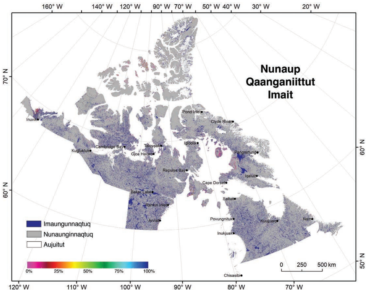
Ajjinguaq 2: Nunannguaq Nunaup Qaangani Imaup Saqqijaarninga Inuit Nunanganni
